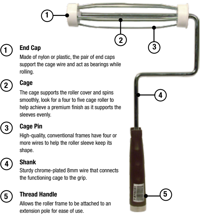
Four Pin Cage Roller
